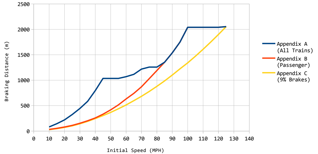
Signalling Braking Distance Data (Level Track)
